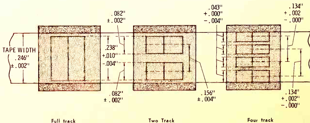
Fig. 3. For proper tracking and interchangeability of tapes, heads should be adjusted to conform to these NAB standard dimensions.
