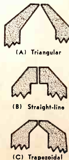
Fig. 2. Basic head-gap configurations.
